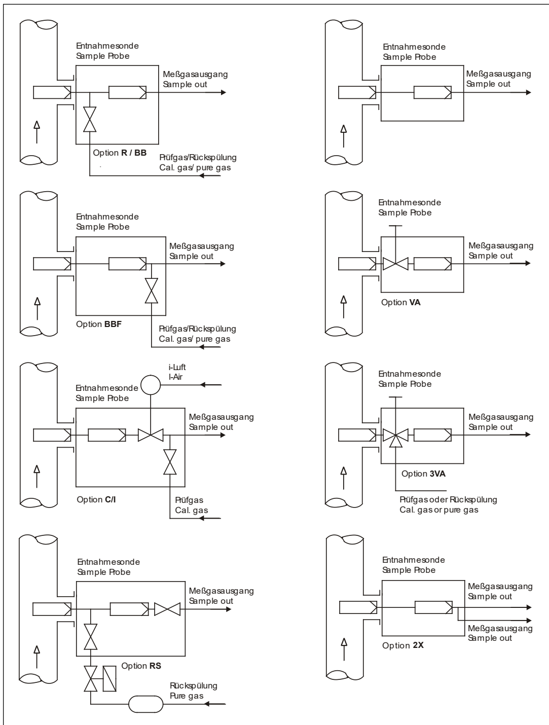
Figure 2 Schematic view of the options for backflush and test gas feeding
