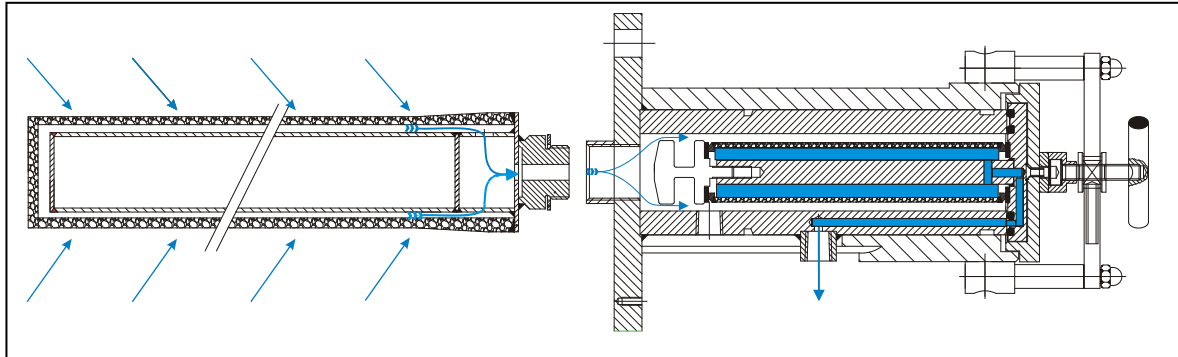
Figure 1 Probe SP3200(V) without options with preliminary filter V20
