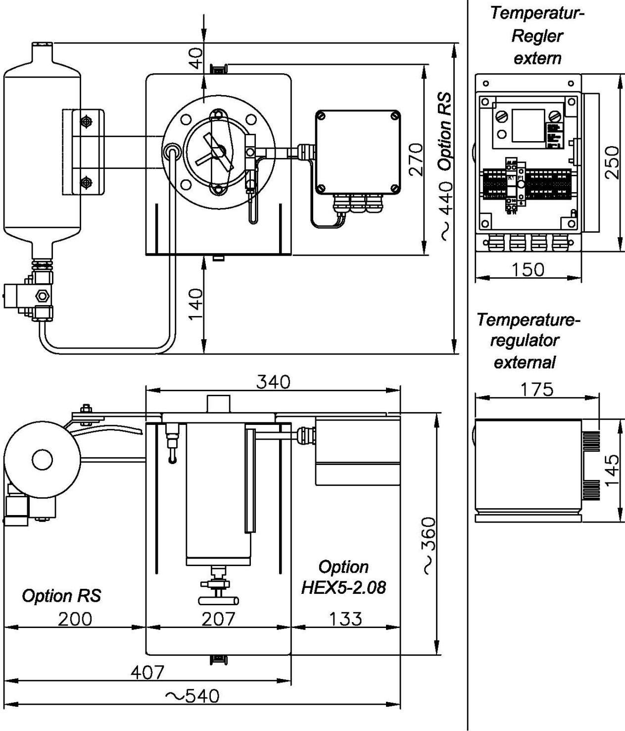
Figure 7 SP3200 RS, HEX5-2.08
